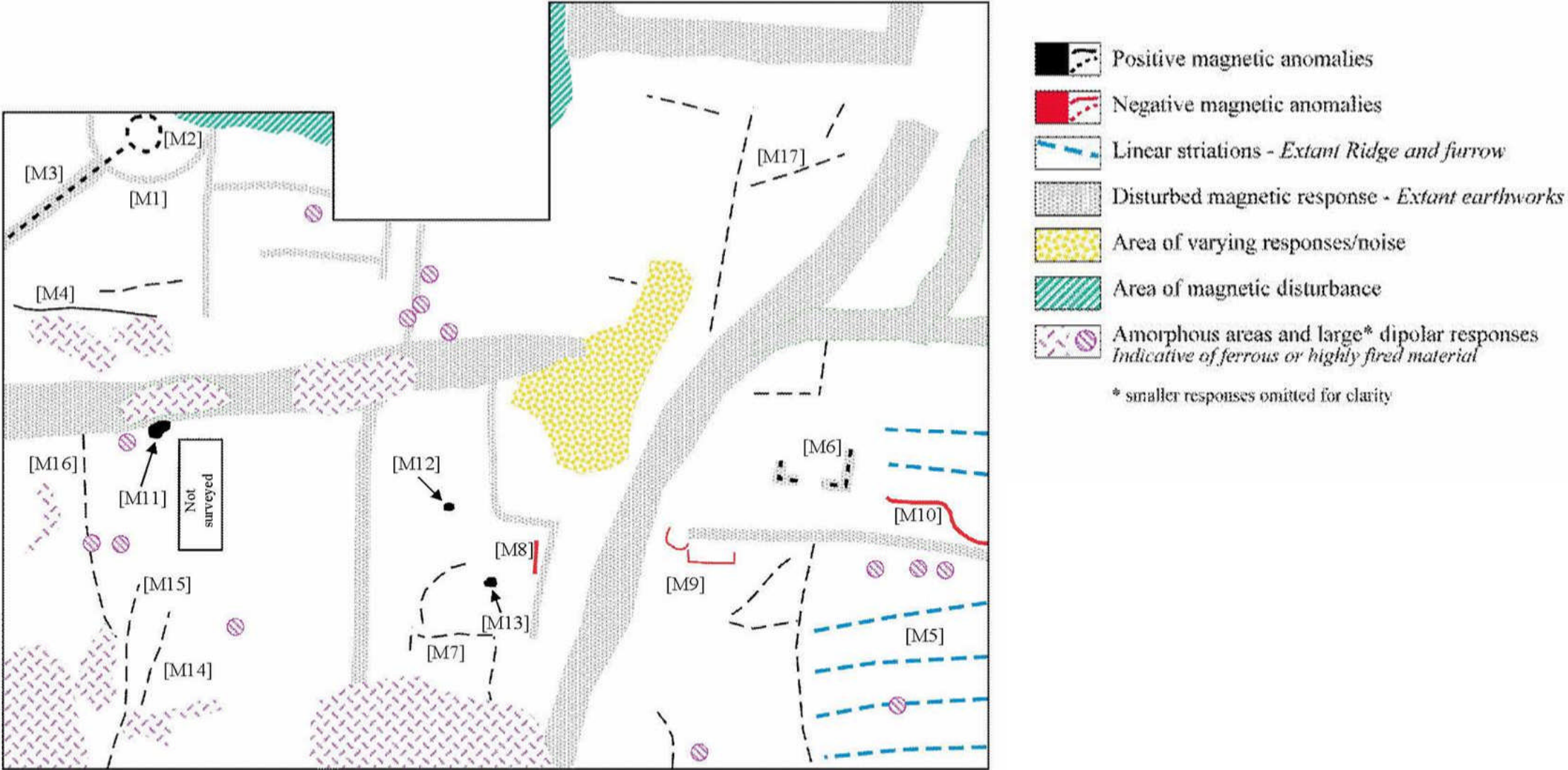
Figure 14 Crow Close - Simplified graphic summary of magnetic data
